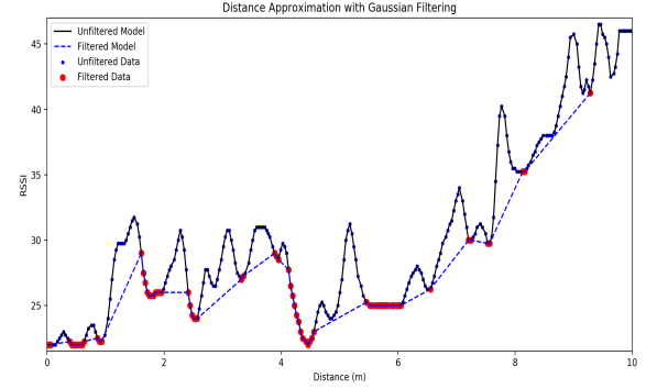
Fig. 5: Gaussian Filtering of Observed RSSI Measurements
